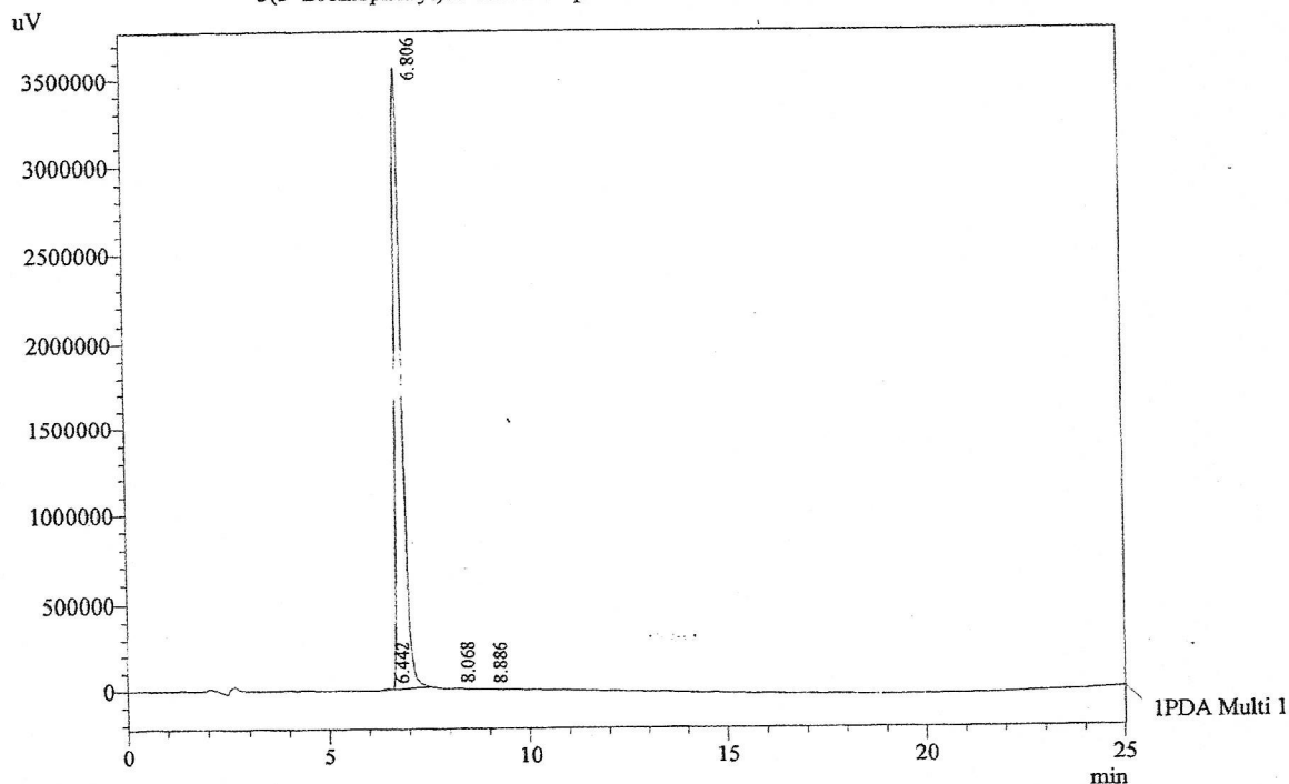
Chromatogram 3(3'-Bromophenyl)coumarin D:\promonence\Data\2013\AUG-2013\1308130.lcd
